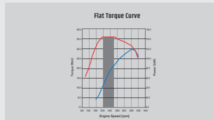
Flat Torque Curve
